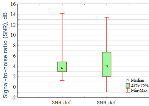
Figure 6. Acoustic emission signal to noise ratio.
