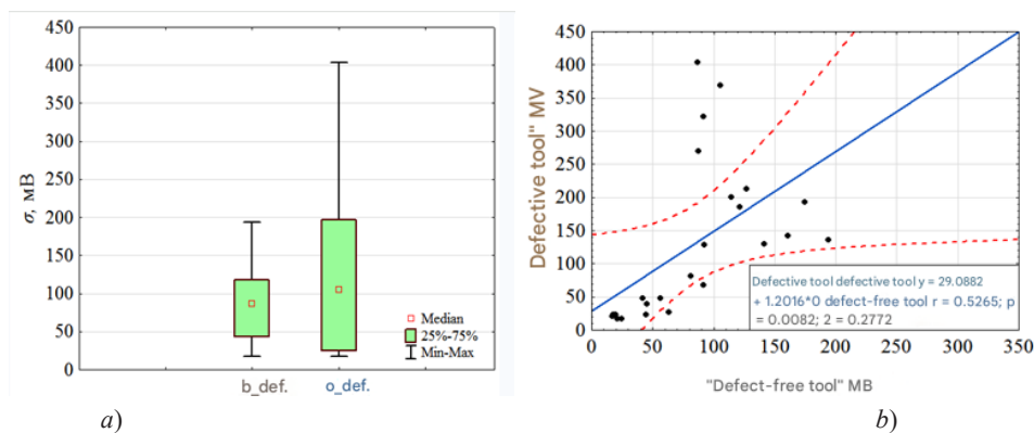
Figure 8. Statistical distinguishability of the parameter \sigma_U : a) Tukey diagram characterizing the variability of the standard deviation of the signal amplitude when testing both instruments ; b) dependence characterizing the increase in the deviation of the signal amplitude when testing a defective instrument.
